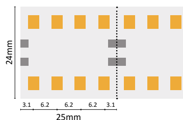
PCB 24mm taglio 25mm/8led - h 1,2mm
