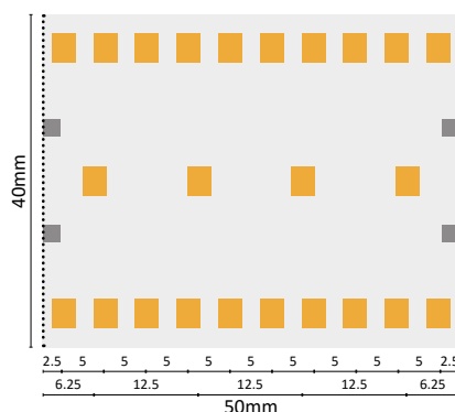
PCB 40mm taglio 50mm/24led - h 1,2mm
