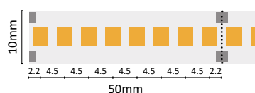
PCB 10mm taglio 50mm/8led - h 1,2mm
